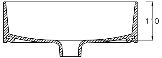
SECTION-VIEW
