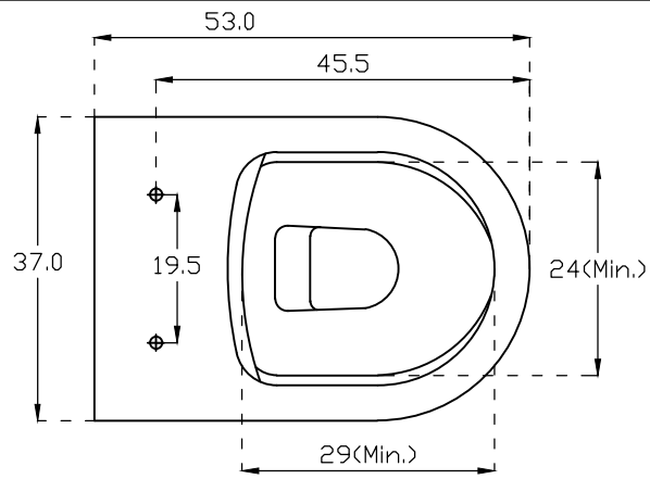
PLAIN VIEW
