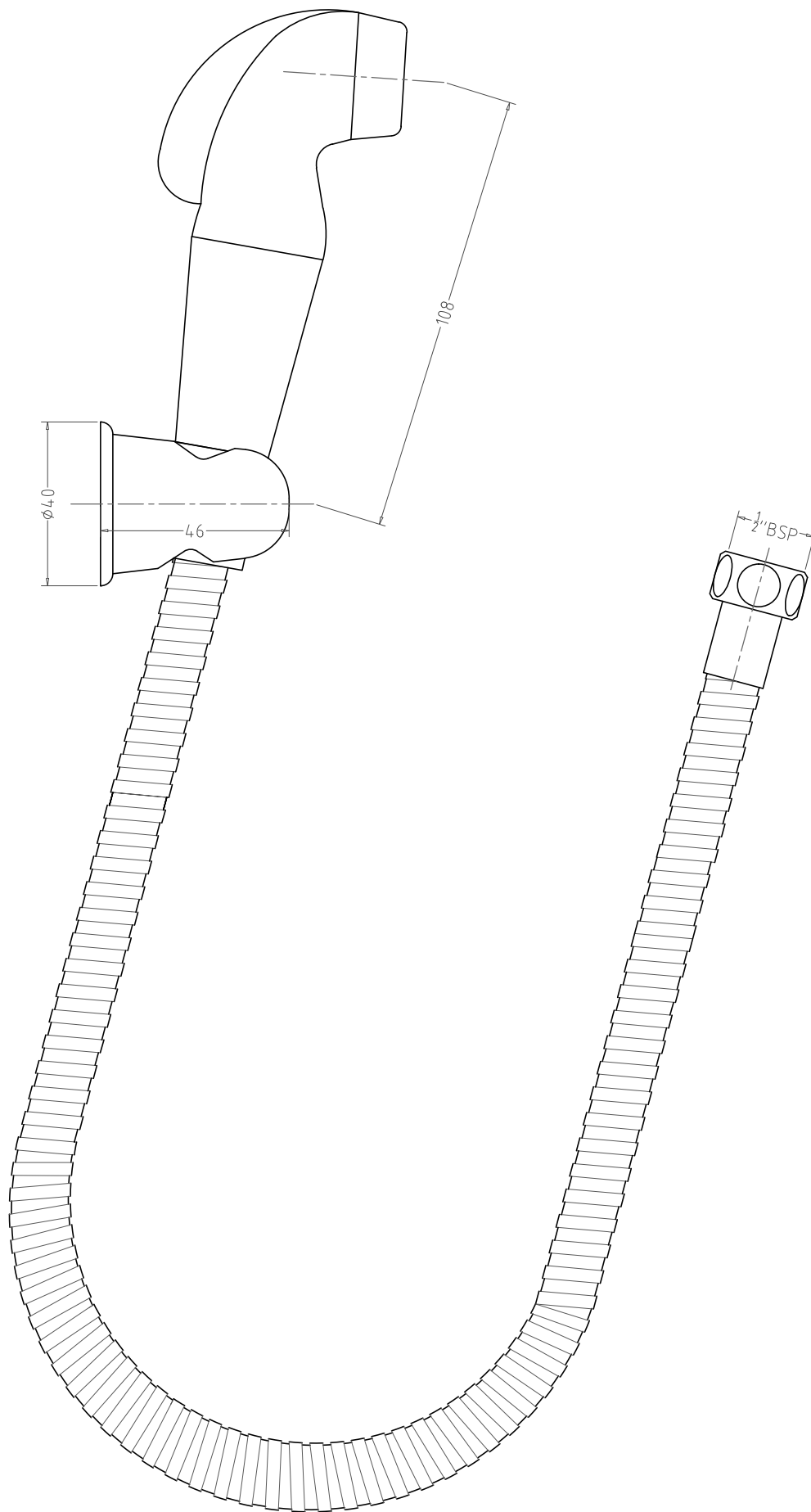
SHOWERS -F160001-HEALTH FAUCETABS WITH DOUBLE LOCK 120 cm S.S. FLEXIBLE HOSE & WALL HOOK
