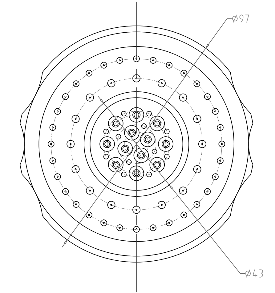
SHOWER-F160008-FIVE FLOW OVER HEAD MASSAGE SHOWER
