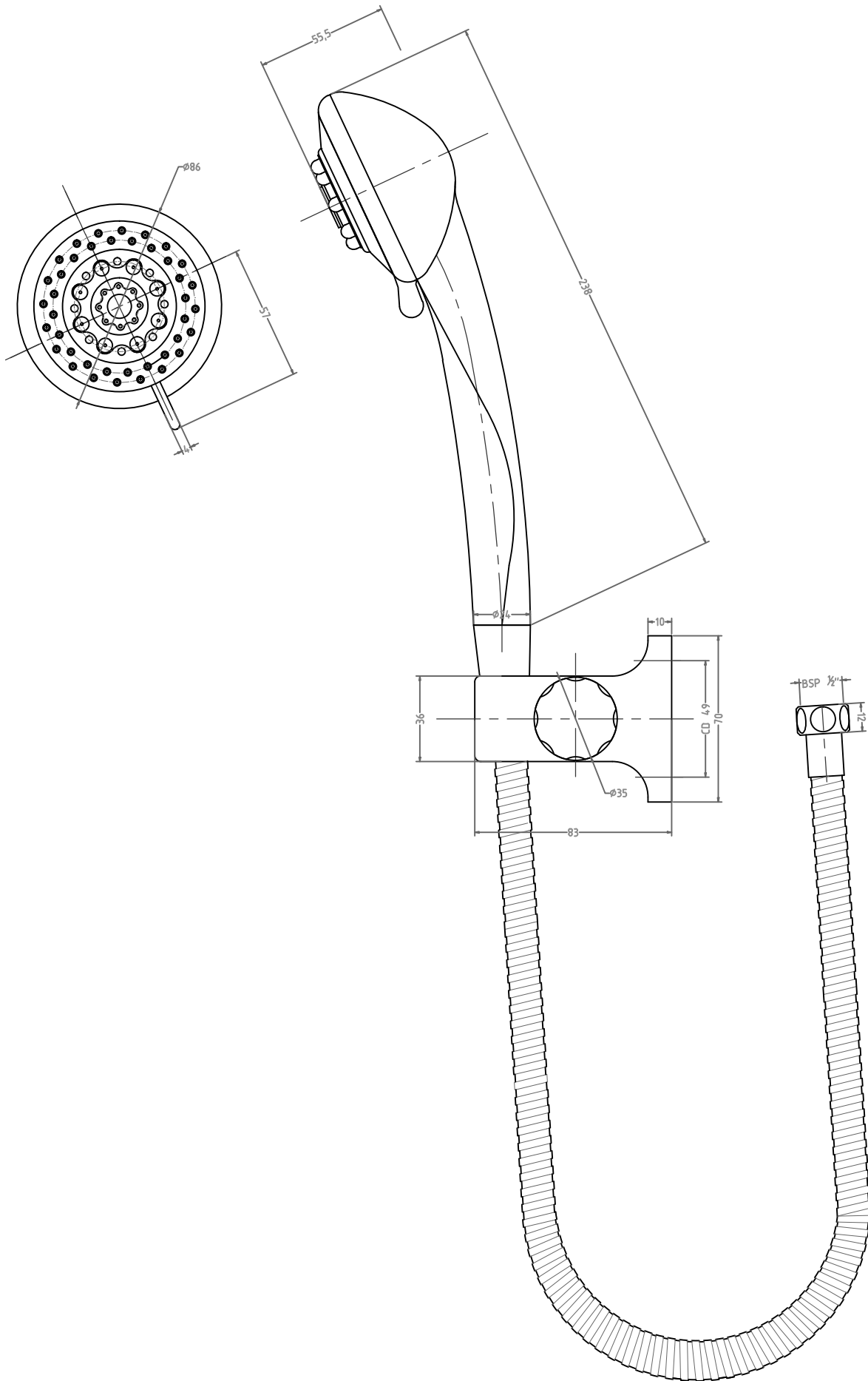
SHOWER-F160009-FIVE FLOW HAND MASSAGE SHOWER WITH DOUBLE LOCK
