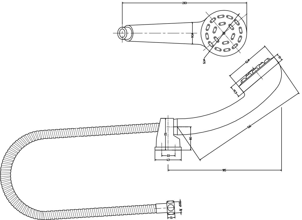
SHOWER-F160026- HAND SHOWER SINGLE FLOW(RUBIT CLEANING SYSTEM) WITH 100CM LONG PVC TUBE & WALL HOOK
