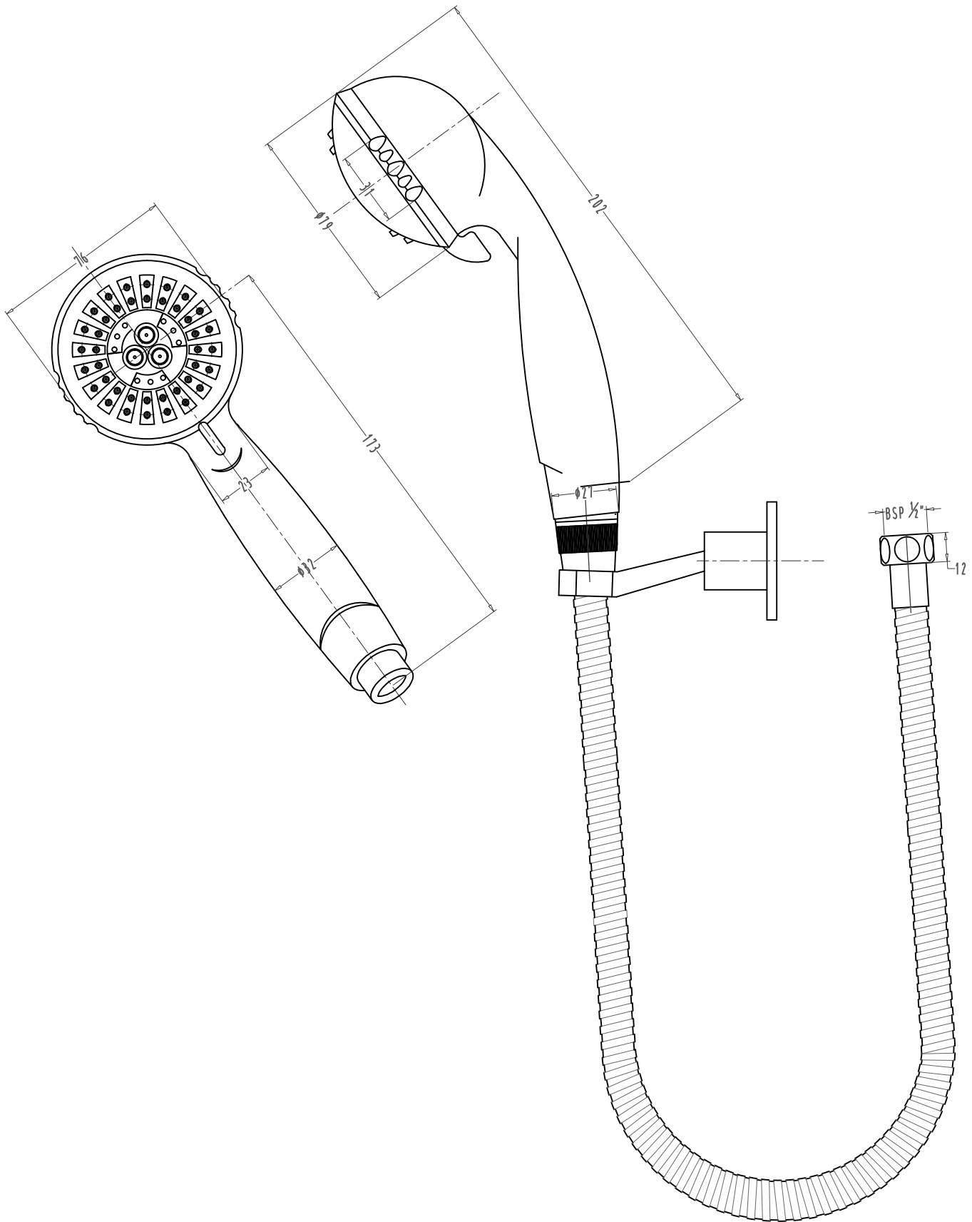
SHOWER- F160046-3 FLOW HAND SHOWER WITH 1.5MCP FLEXIBLE TUBE WITH HOOK DATE-22.01.16
