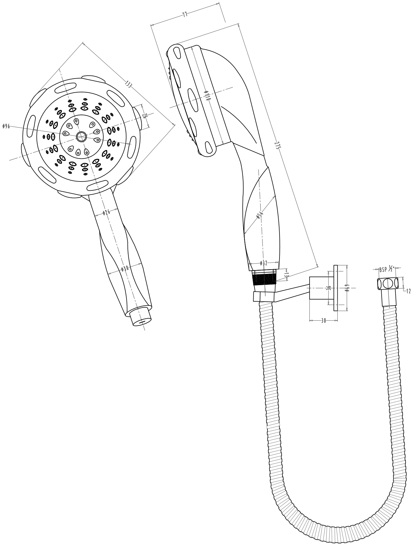
SHOWER- F160056-LED HAND SHOWER WITH 1.5MCP FLEXIBLE TUBE WITH HOOK DATE-22.01.16
