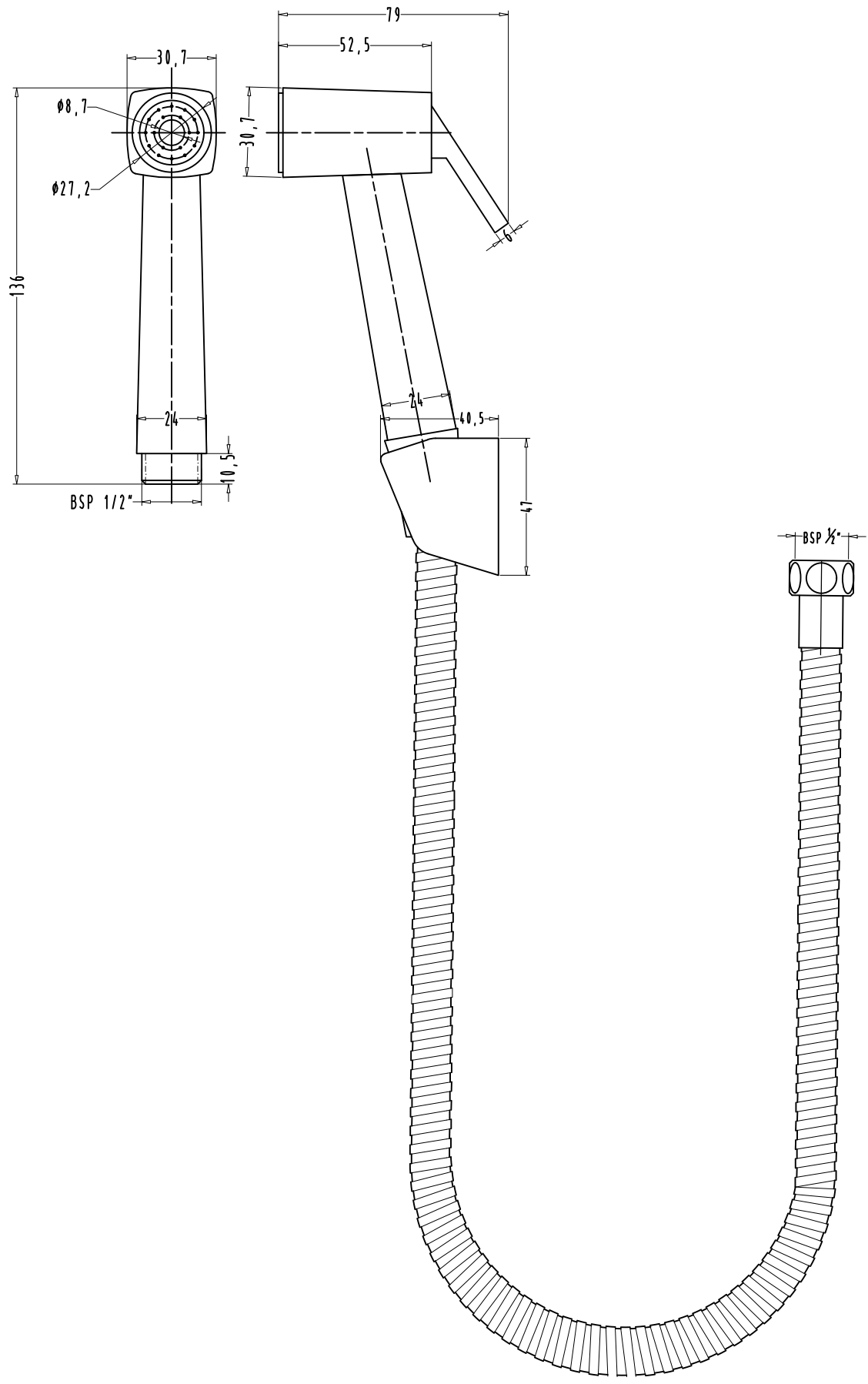
F160109- GEM HF WITH 1.2Mtr. HOSE PIPE & HOOK
