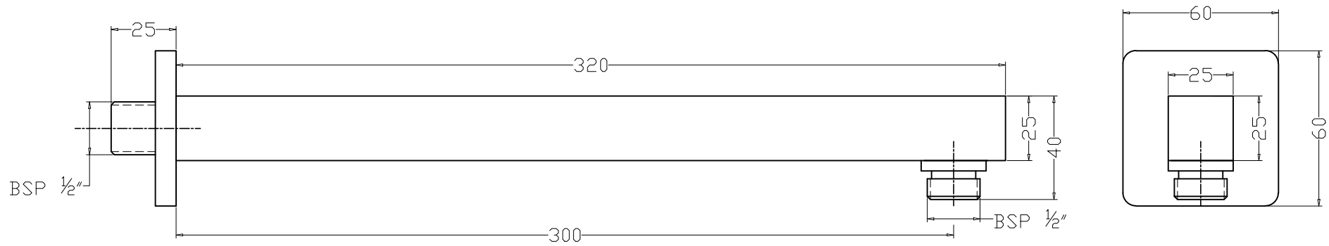
SHOWER ACCESSORIES-F160117 -SHOWER ARM 300mm SQUARE WITH FLANGE
