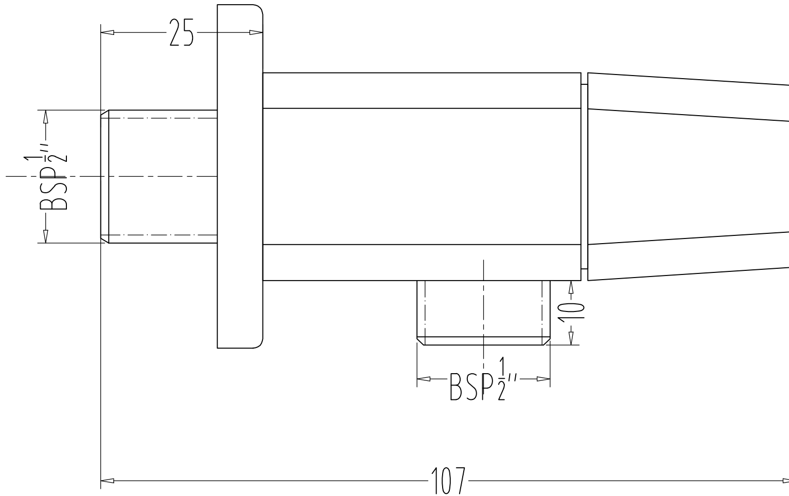
ARMADA F260004 ANGULAR STOP COCK WITH WALL FLANGE
