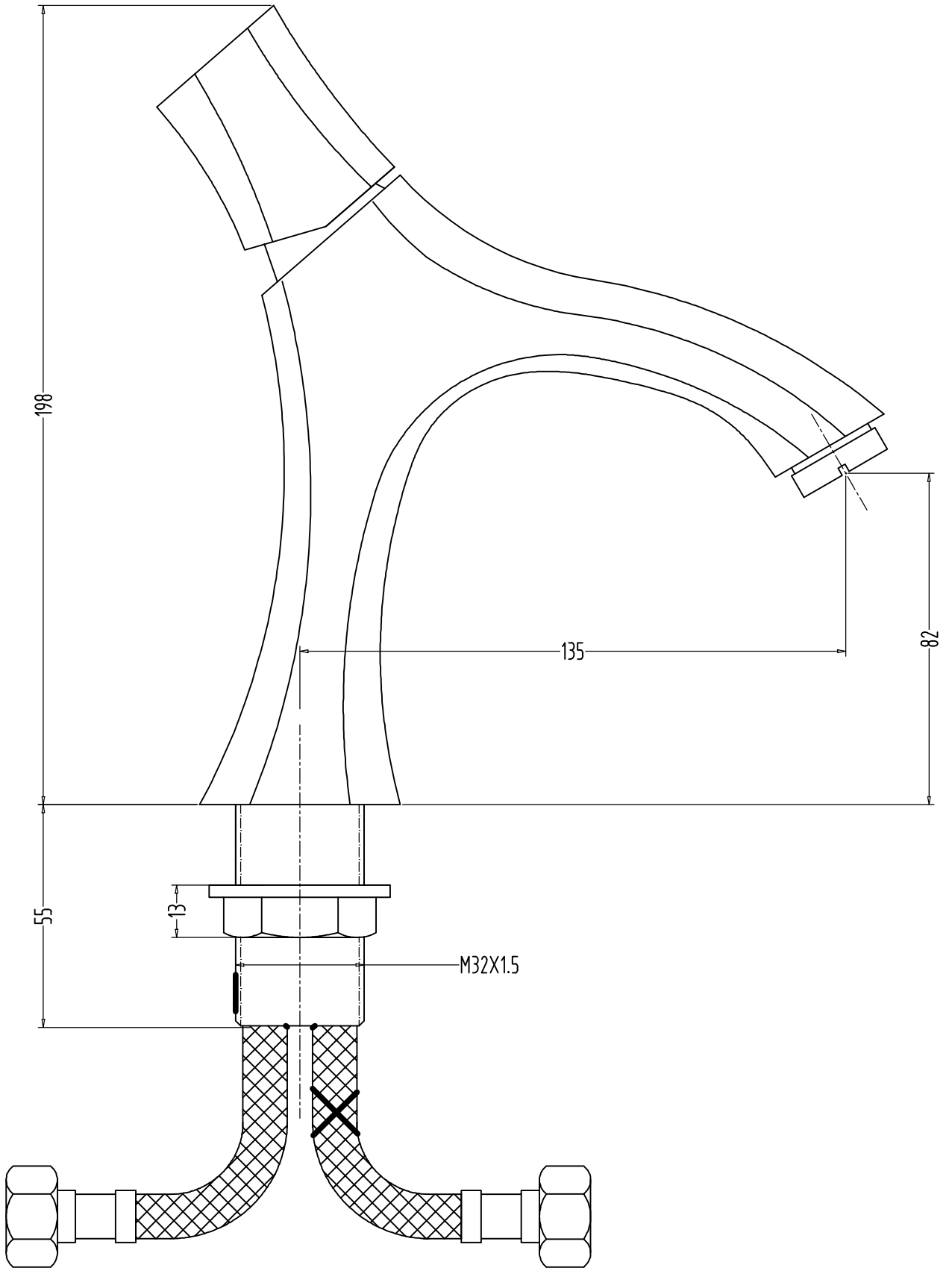
ARMADA F260009 S/L BASIN MIXER
