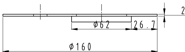
WALL FLANGE WITH 'O'RING
