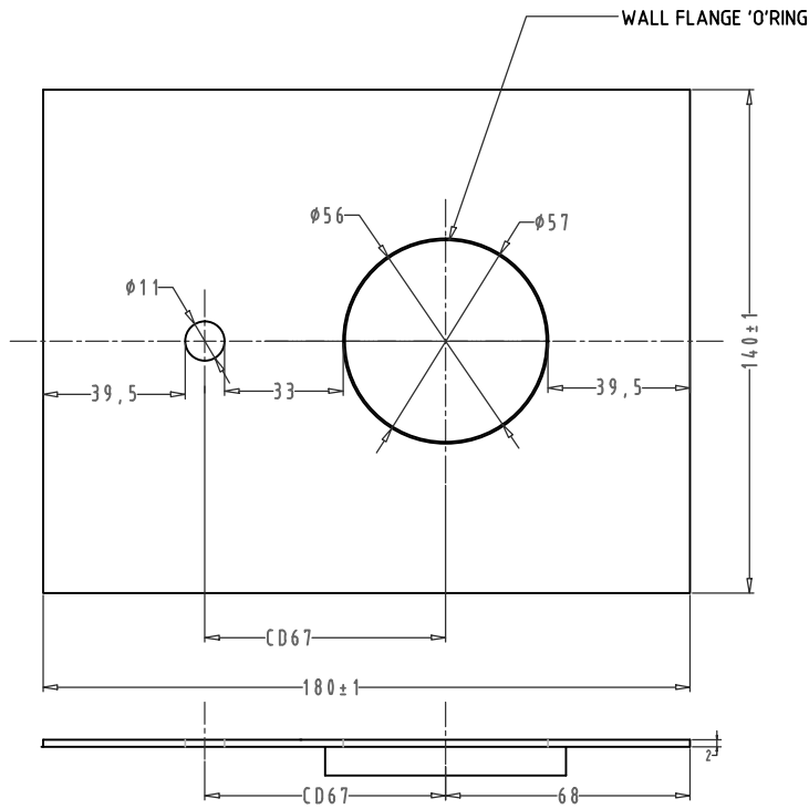
WALL FLANGE WITH 'O'RING
