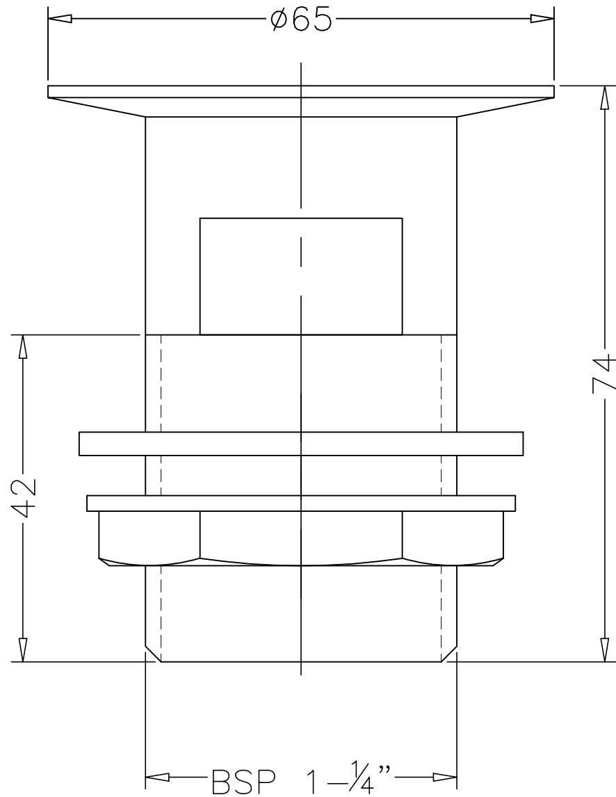
F850023 - WASTE COUPLING 32 mm. ECONOMY MODEL( HALF THREAD)
