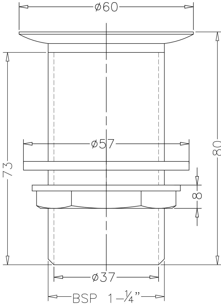
F860010 - SS WASTE COUPLING 32 mm. ( FULL THREAD)
