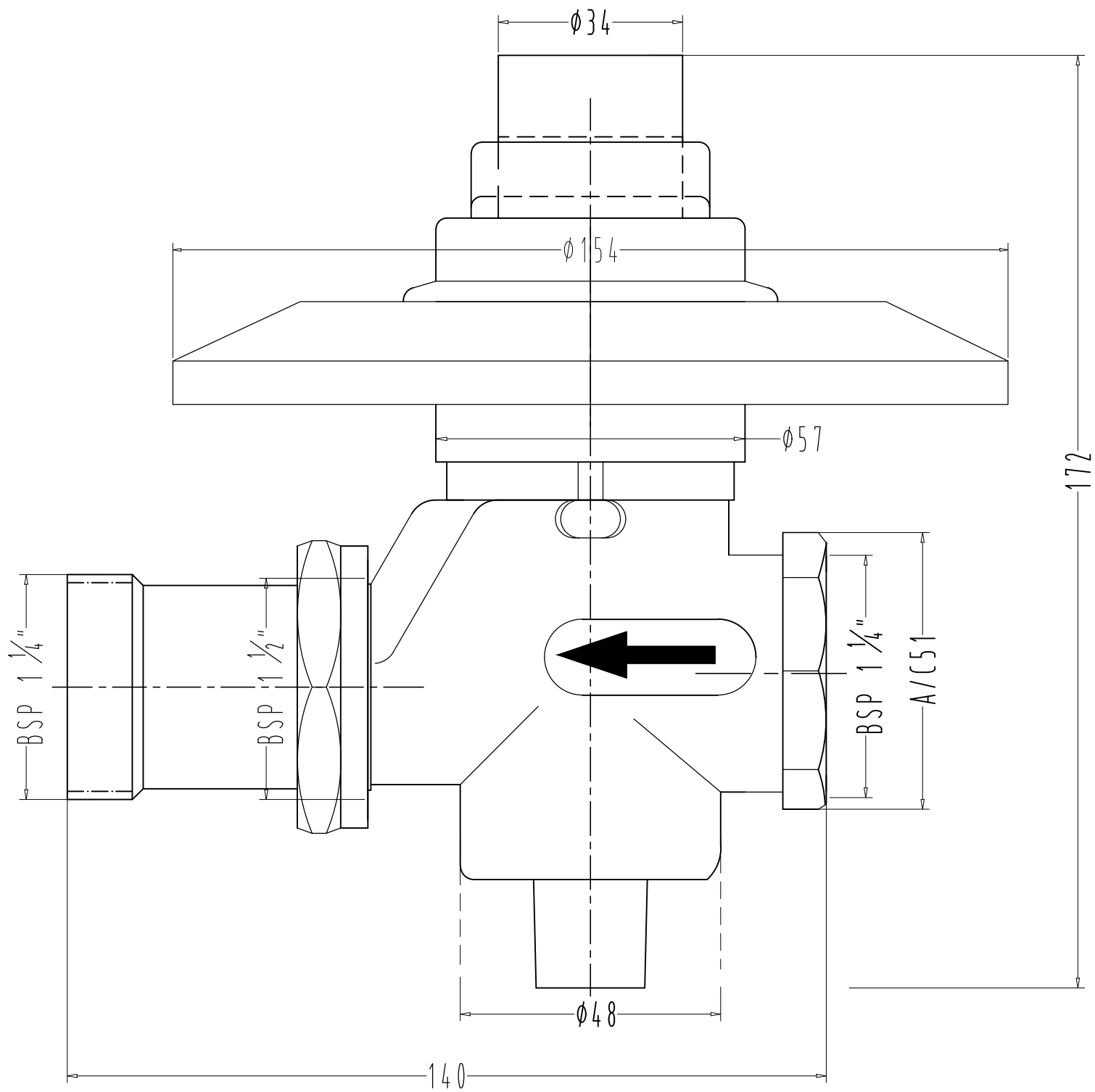
F860035CP-FLUSH VALVE DUAL FLOW 32 MM CONCEALED NEO
