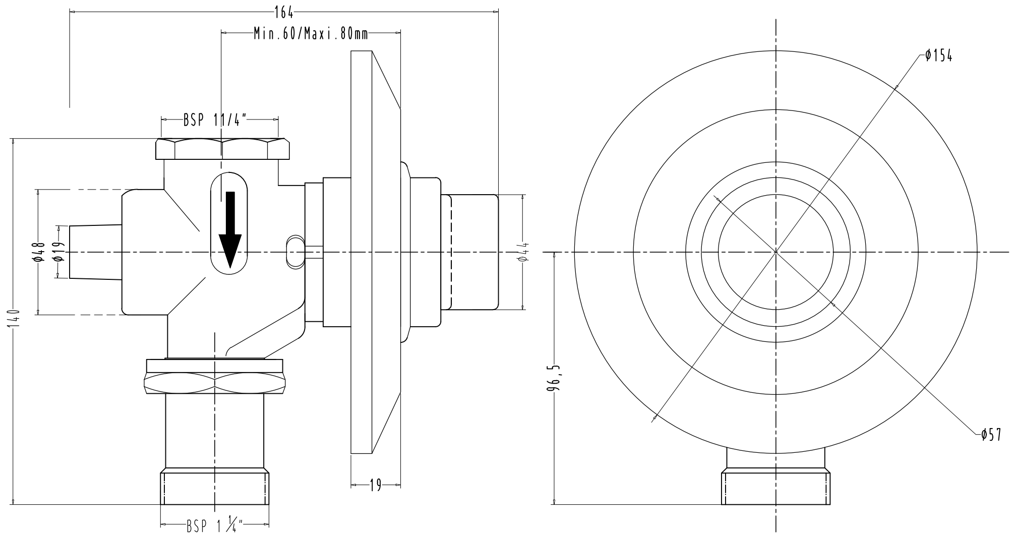
F860037CP-NEO FLUSH VALVE 32 MM SINGLE FLUSH (ROUND)
