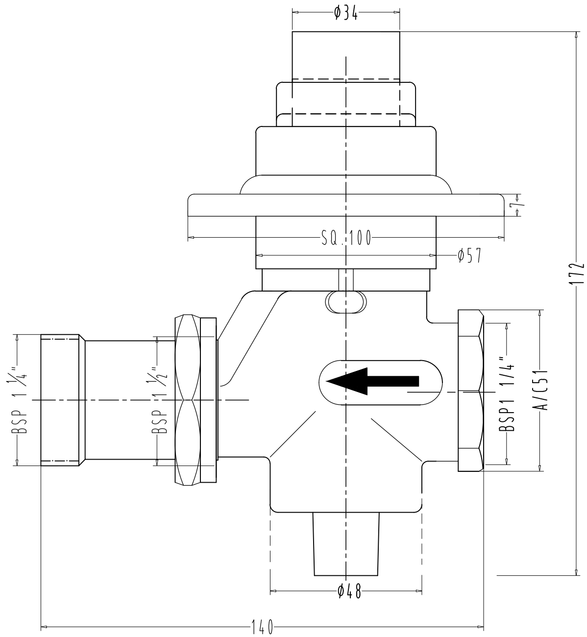
F860038CP-FLUSH VALVE 32 MM DUAL FLUSH WITH SQUARE PLATE
