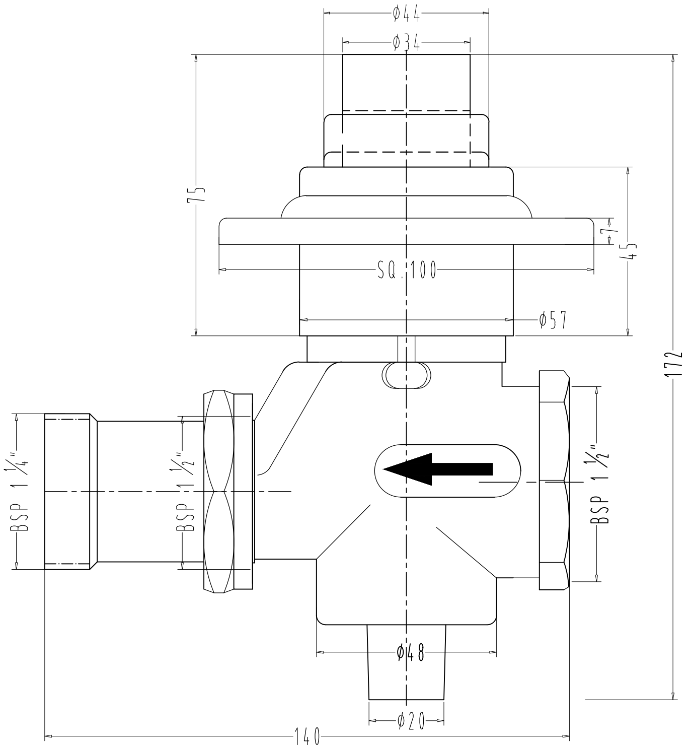
ADDONS:F860042CP-FLUSH VALVE 40 MM DUAL FLUSH WITH SQUARE PLATE NEO
