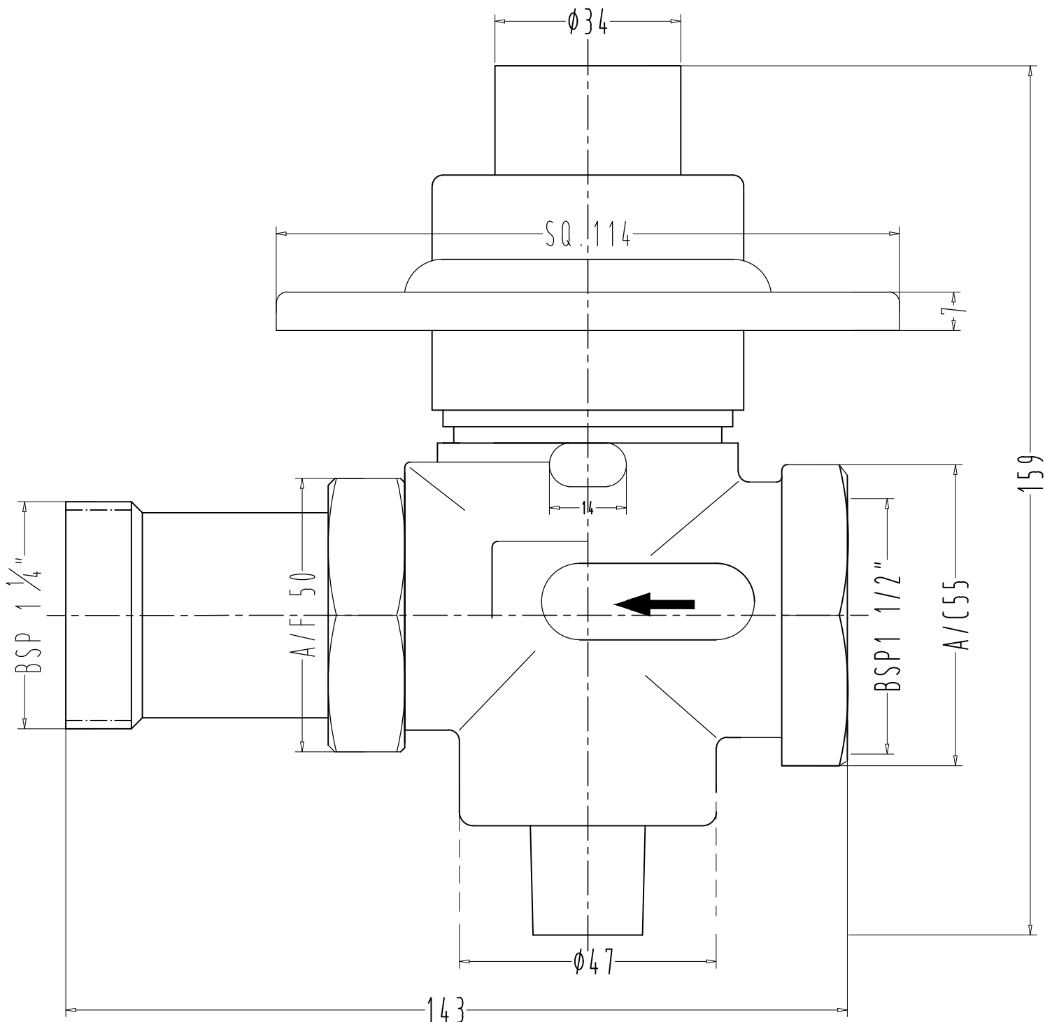
F860043CP-FLUSH VALVE 40 MM SINGLE FLUSH SQUARE PLATE
