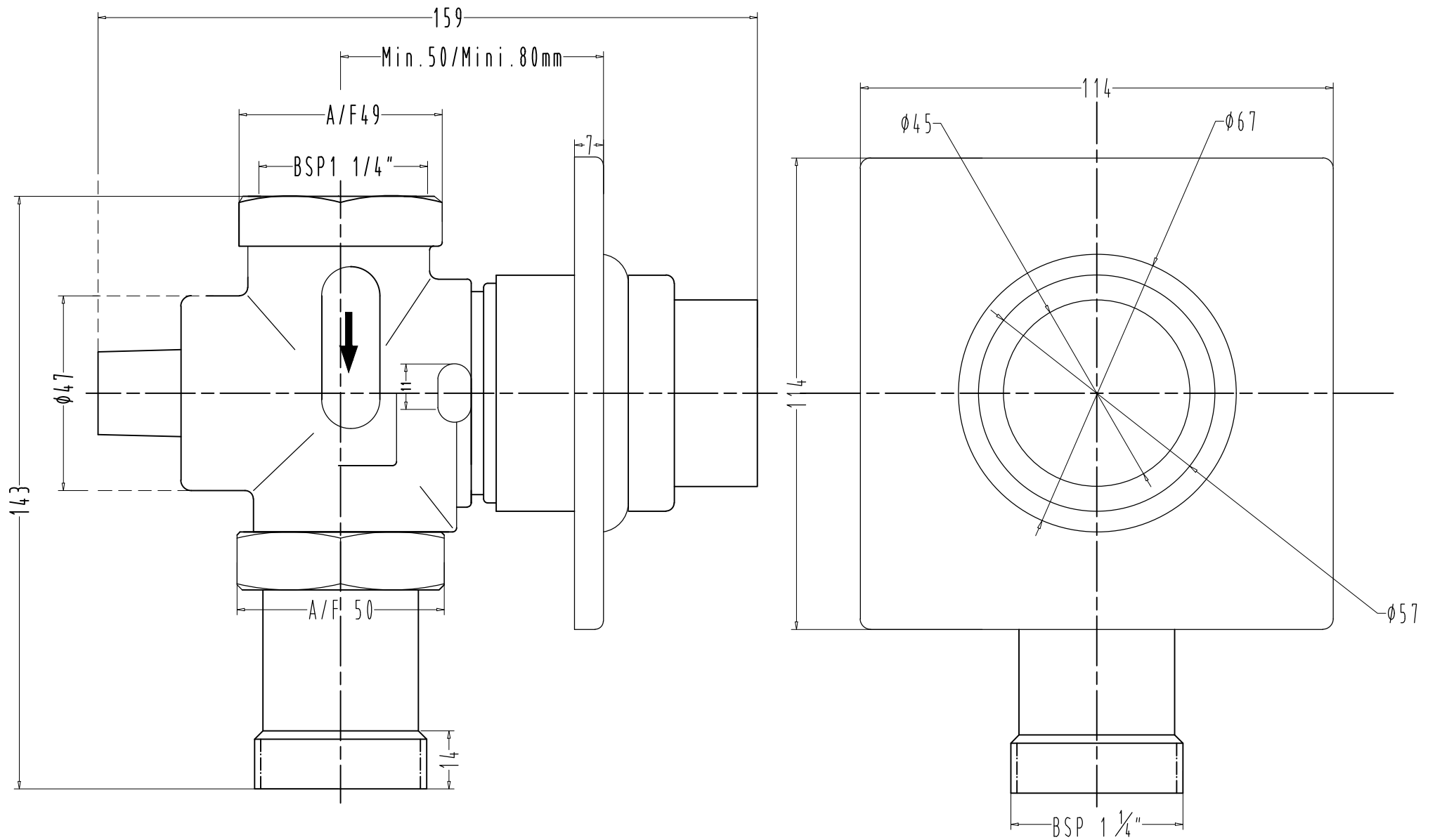
F860045P-PLUS CONCEALED FLUSH VALVE 32 MM SINGLE FLUSH SQUARE PLATE
