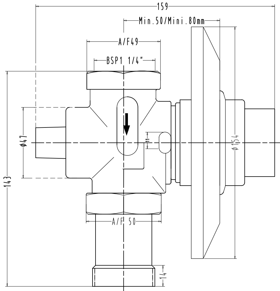
F860046P-PLUS CONCEALED FLUSH VALVE 32 MM SINGLE FLUSH ROUND PLATE
