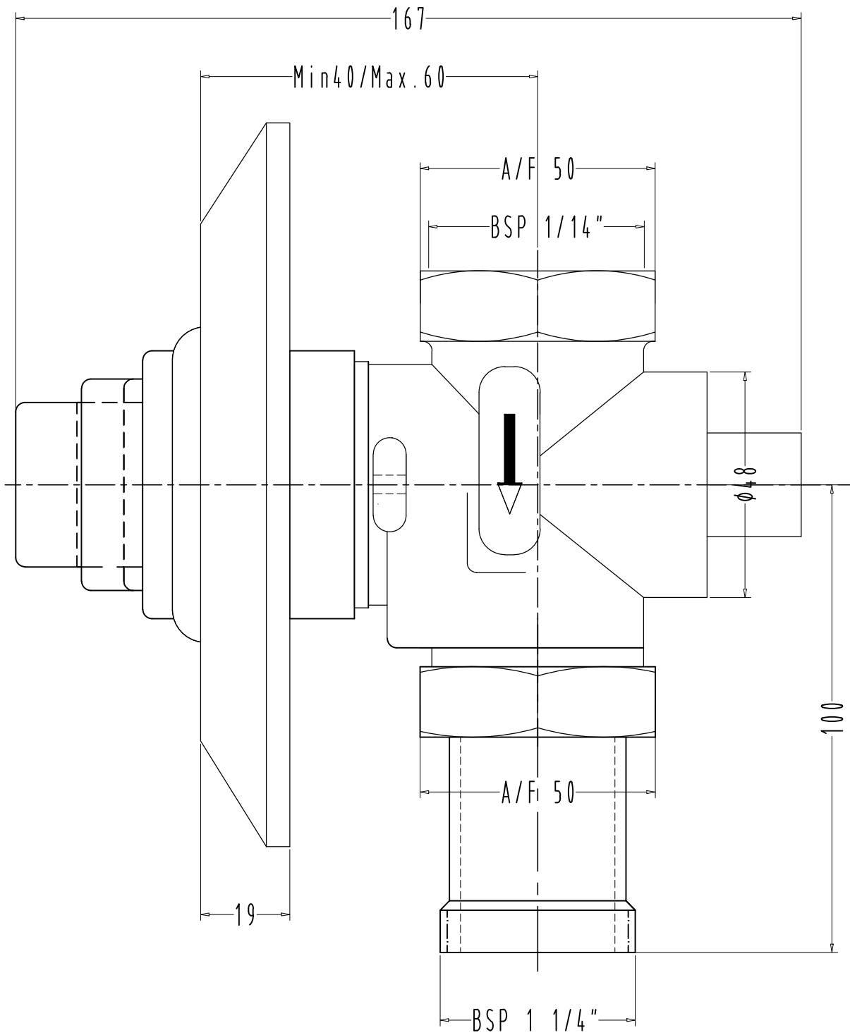
ADDONS -F860047-PLUS CONC FLUSH VALVE 32 MM DUAL FLUSH WITH ROUND PLATE
