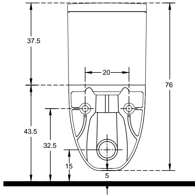
BACK VIEW
