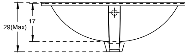
FRONT ELEVATION
