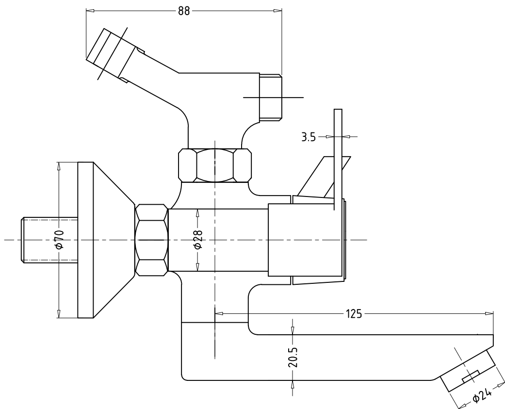
ASPIRO: F570018 WALL MIXER TELEPHONIC WITH CRUTCH
