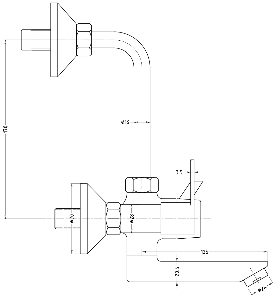
ASPIRO: F570020 WALL MIXER WITH L BEND
