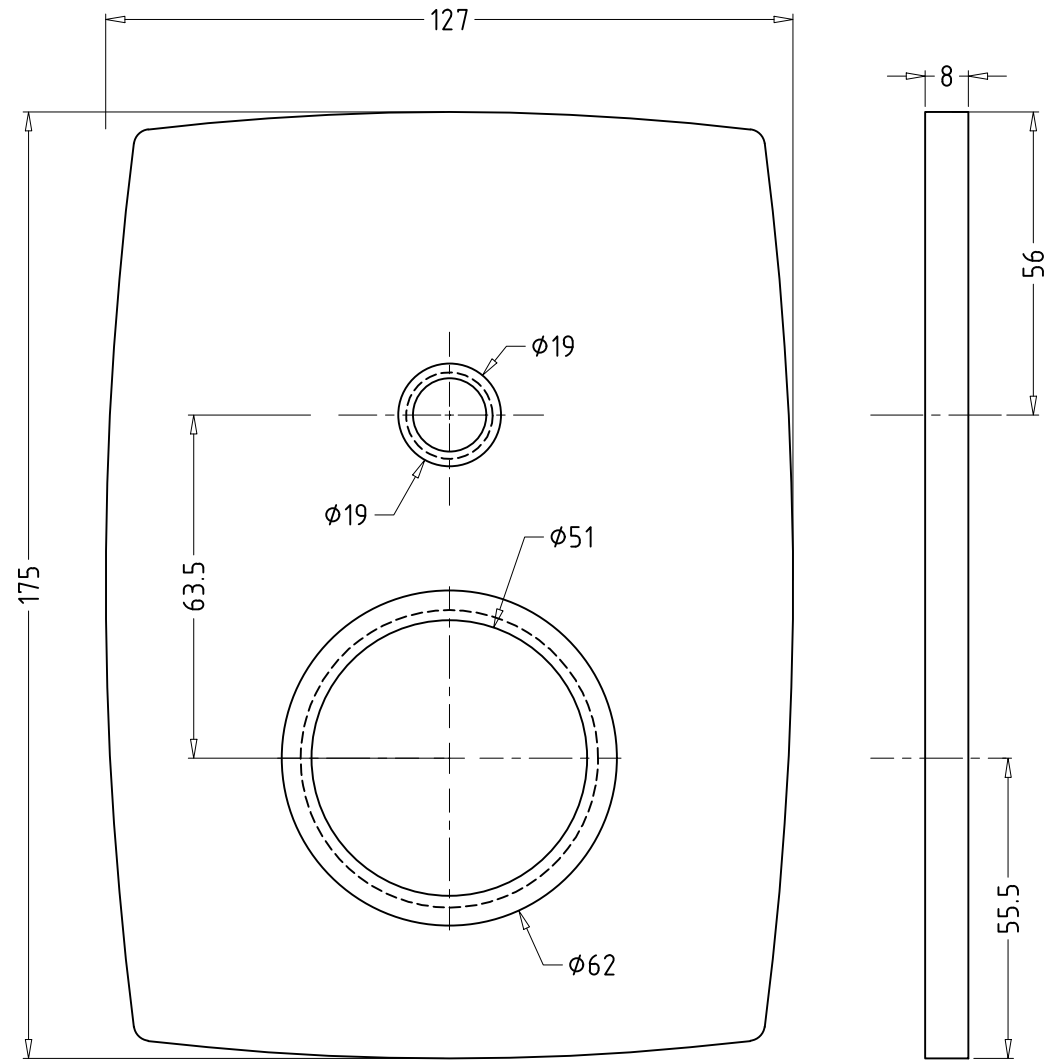
ASPIRO : SL DIVERTOR NORMAL PLATE
