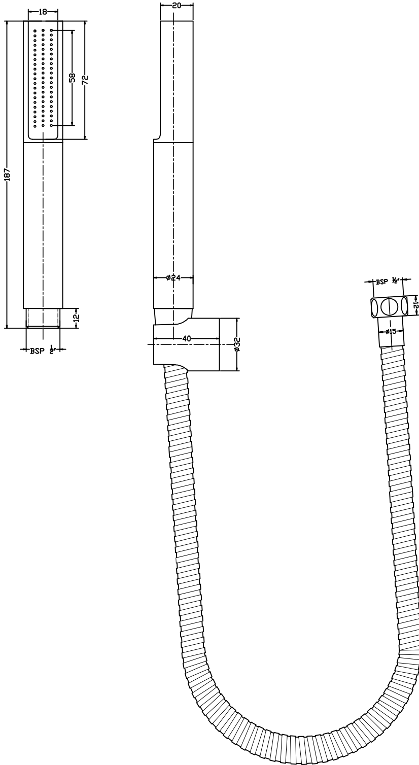
HAND SHOWER- F160150 RGD HAND SHOWER WITH 1.5M HOSE PIPE & HOOK (RGD)
