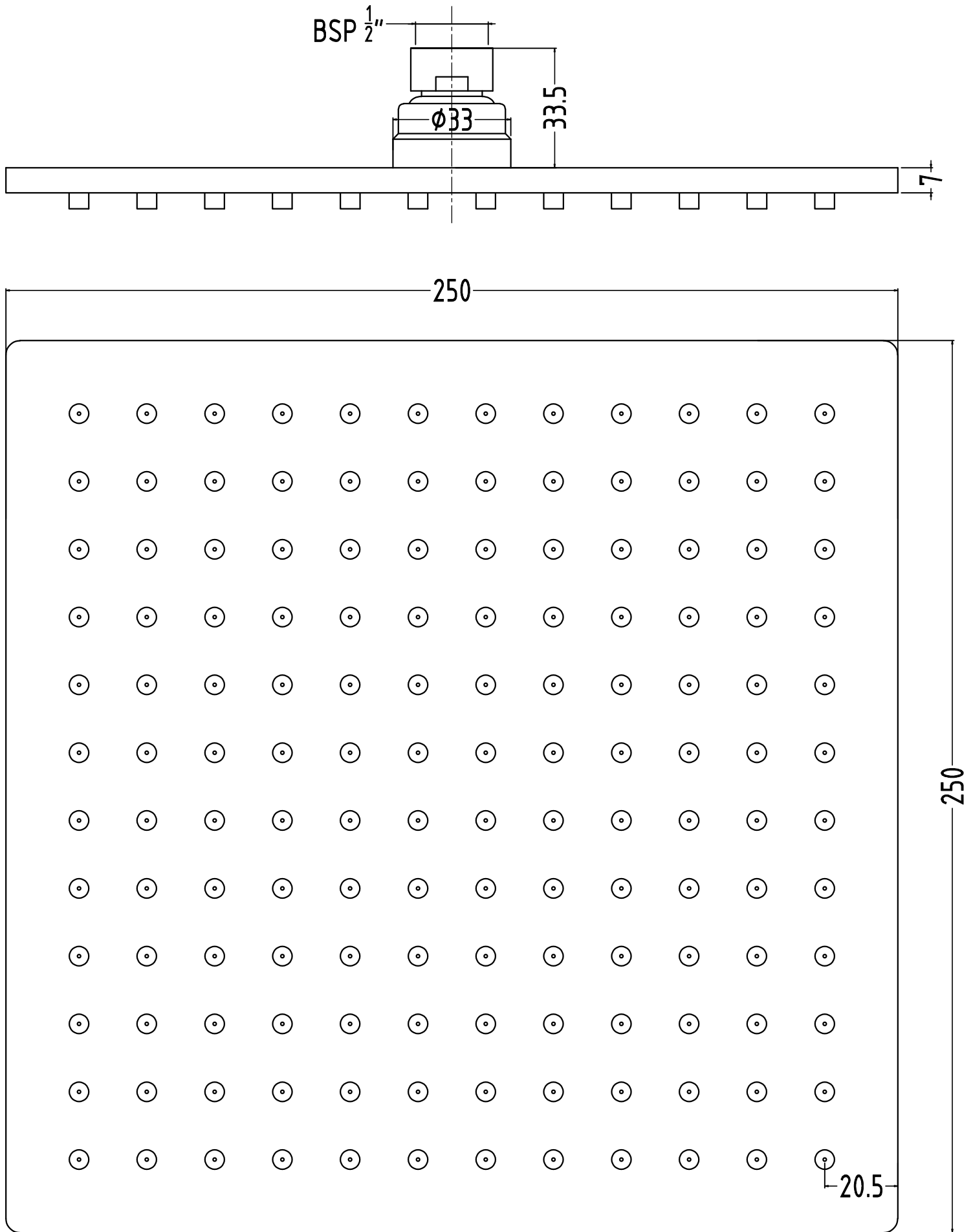
HUSE-GOLD SHOWER CAT.No. : F160161 PGD SHOWER 250x250 MM SQUARE
