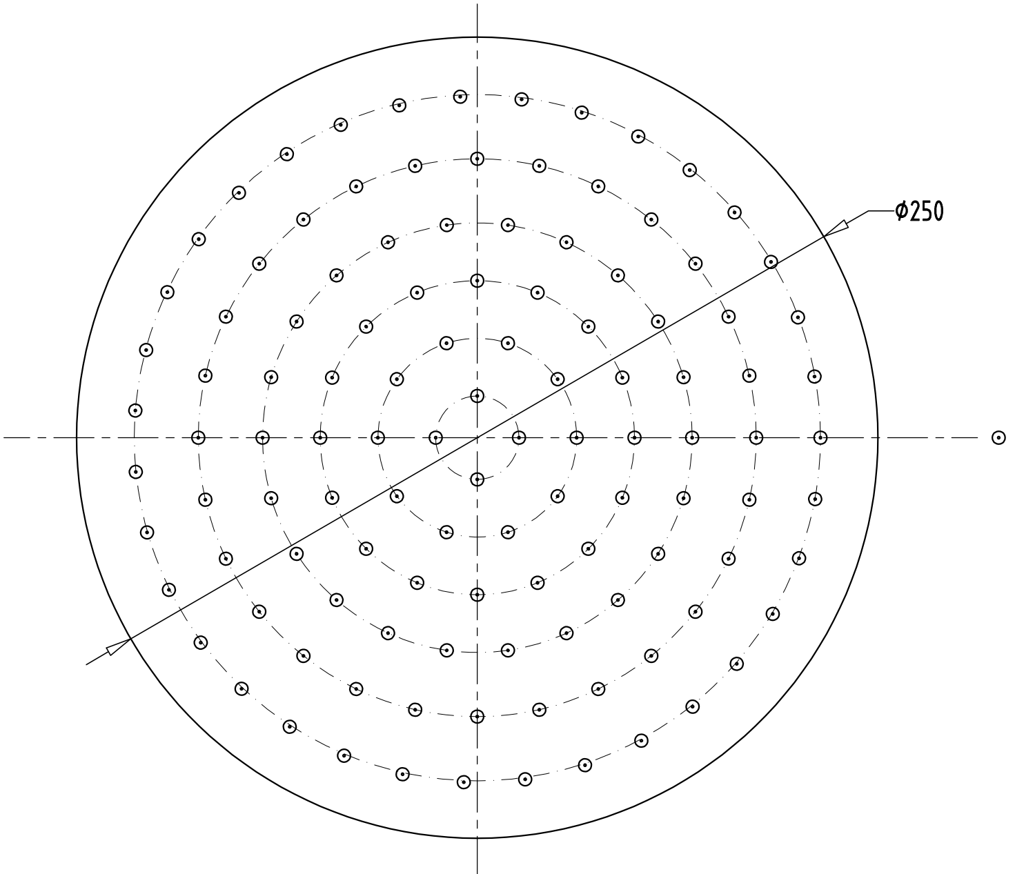
HUSE-GOLD SHOWER CAT.No.: F160162 PGD SHOWER 250 MM ROUND
