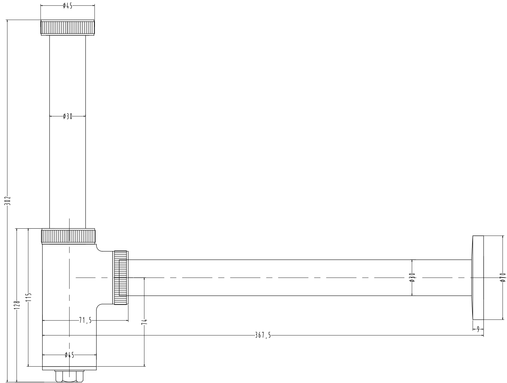
F850004 - BOTTLE TRAP PREMIUM 32MM WITH 300MM & 190MM LONG WALL CONNECTION PIPE AND WALL FLANGE
