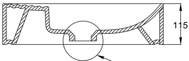
SECTIONAL VIEW
