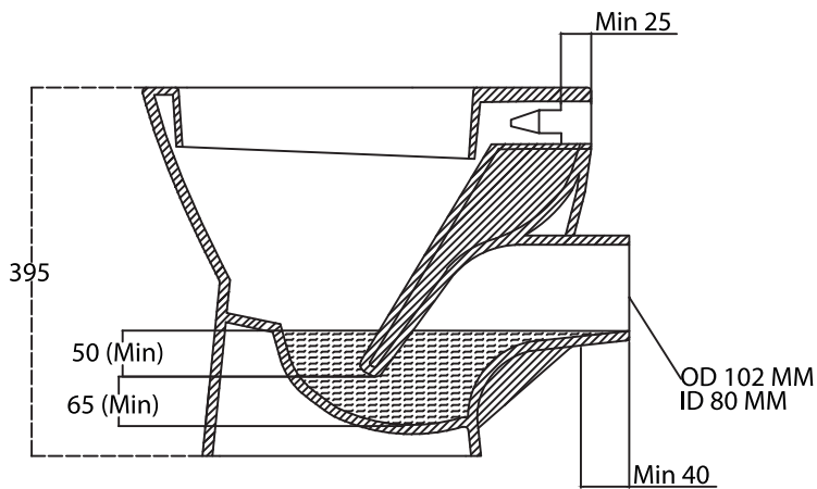
SECTIONAL VIEW
