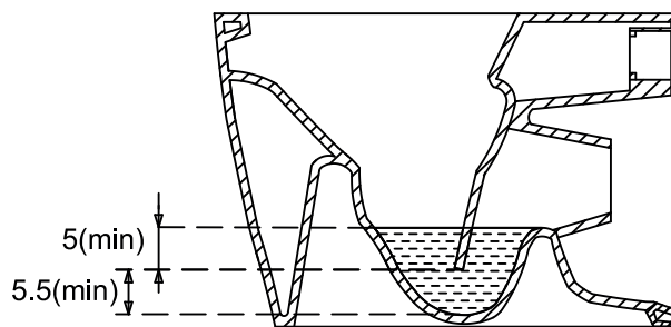
SECTIONAL VIEW
