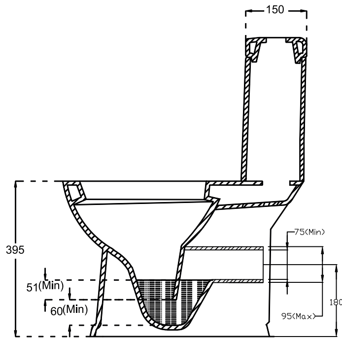
SECTIONAL VIEW
