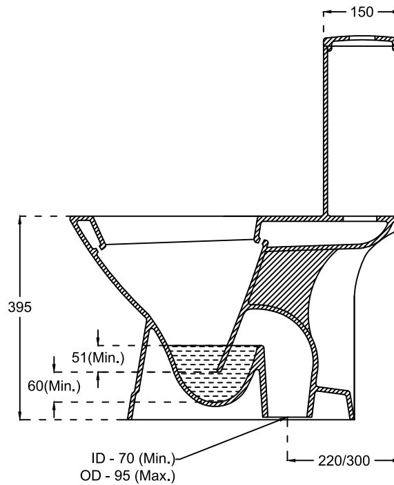
SECTION-VIEW
